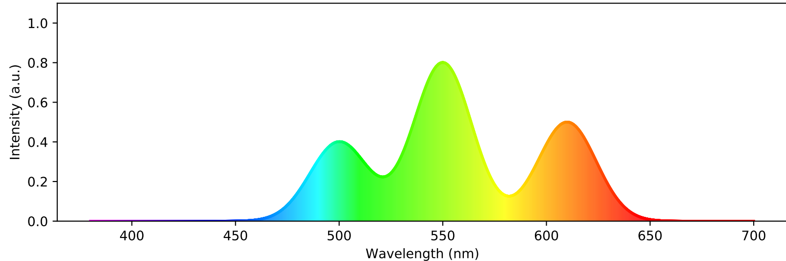
Emission Spectrum in Tube A
