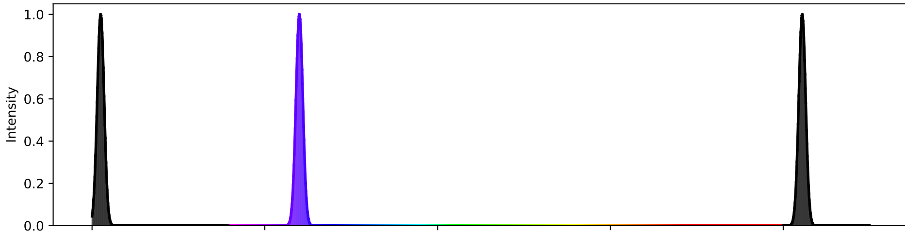
Mercury Emission Spectrum
