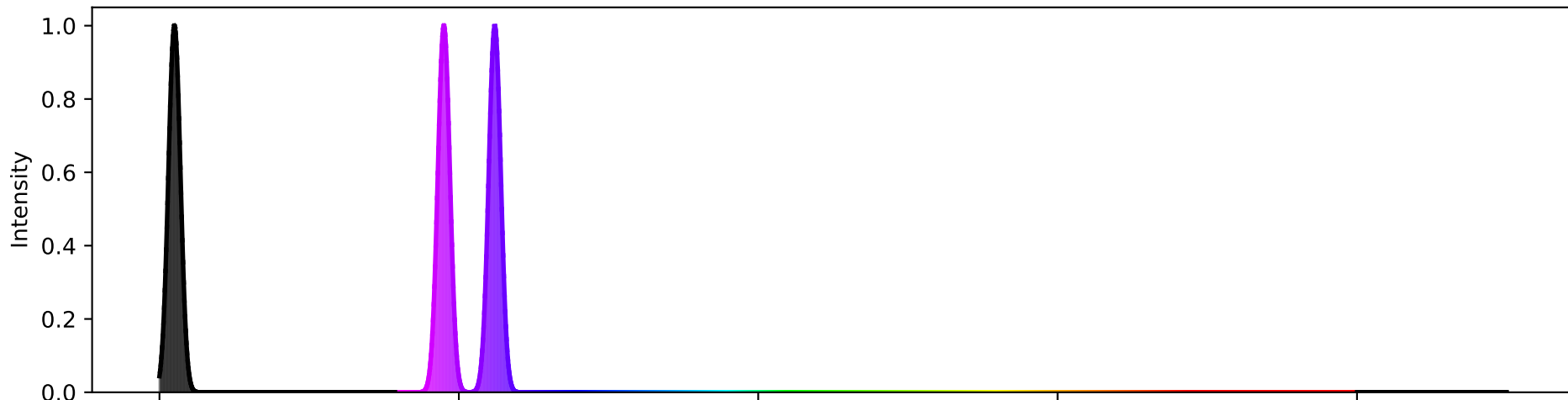
Argon Emission Spectrum
