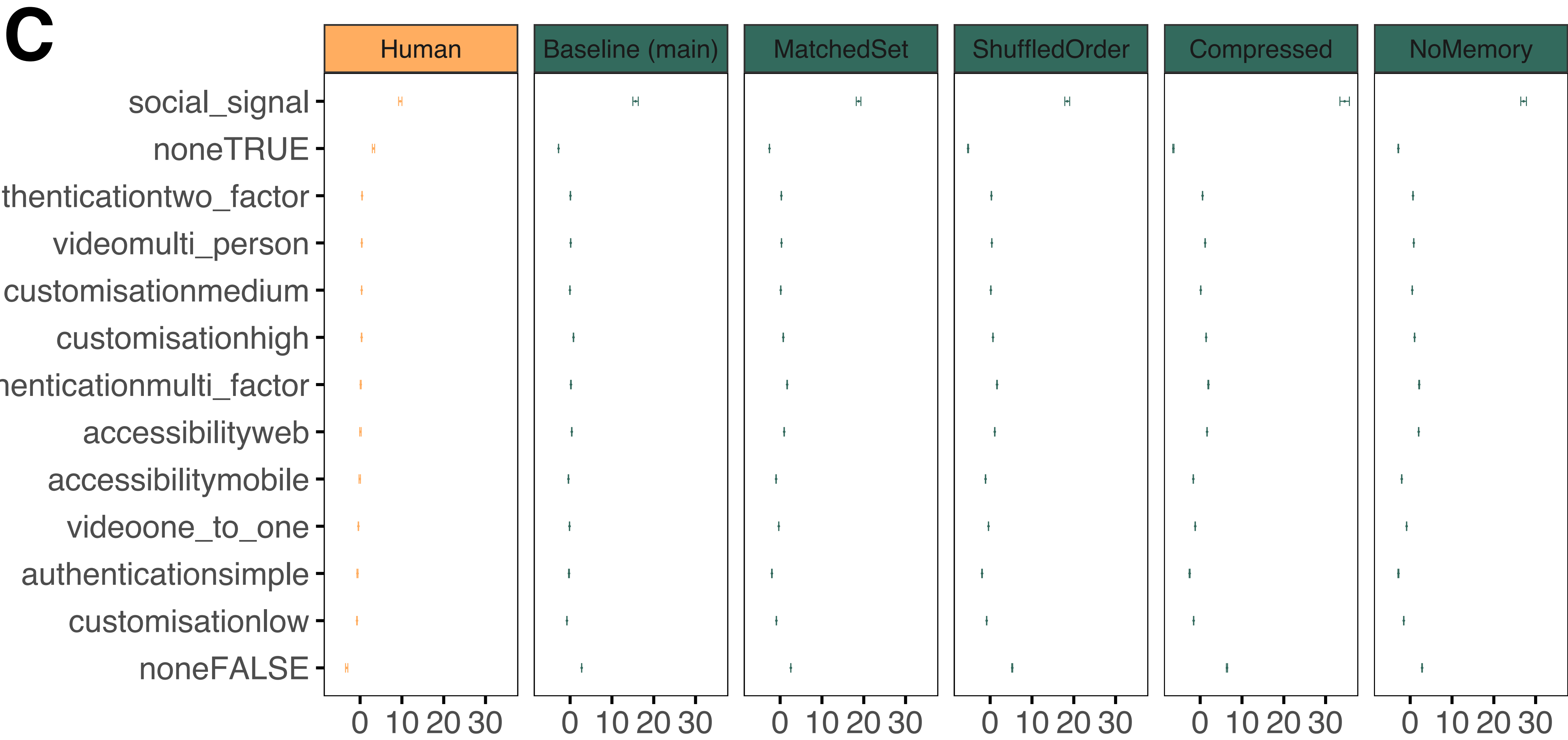
Average partworth utility (GPT5, by prompt variant, 95% CI)
