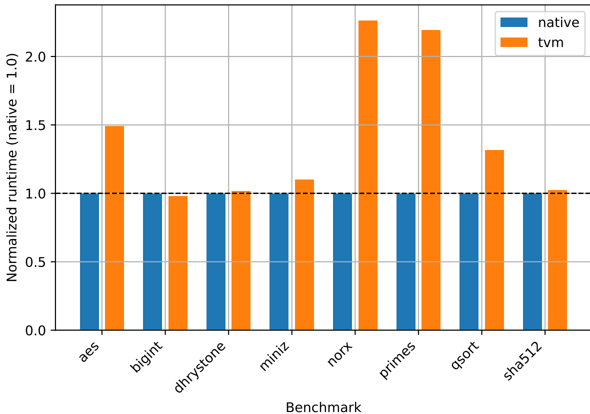
RV8 benchmarks. Native Linux vs. TVM Linux
