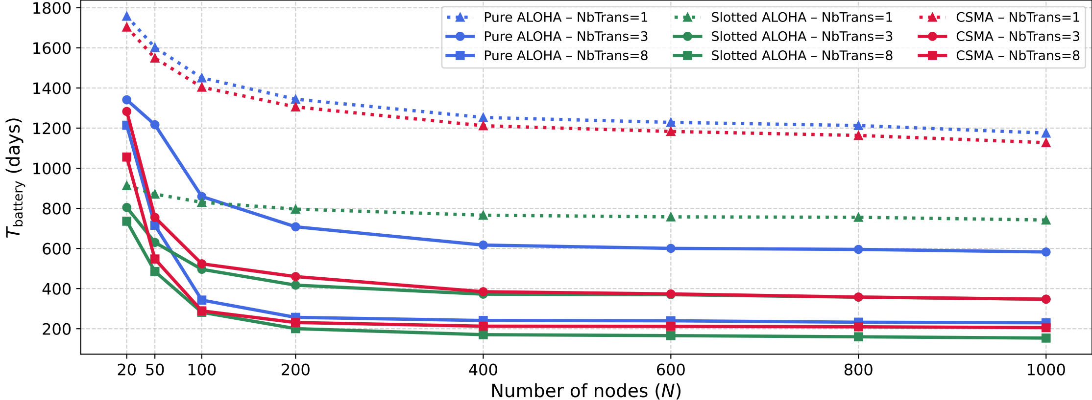
Estimated battery lifetime T_{\text{battery}} — Pure ALOHA vs Slotted ALOHA vs CSMA, Confirmed (NbTrans = 1 / 3 / 8)
