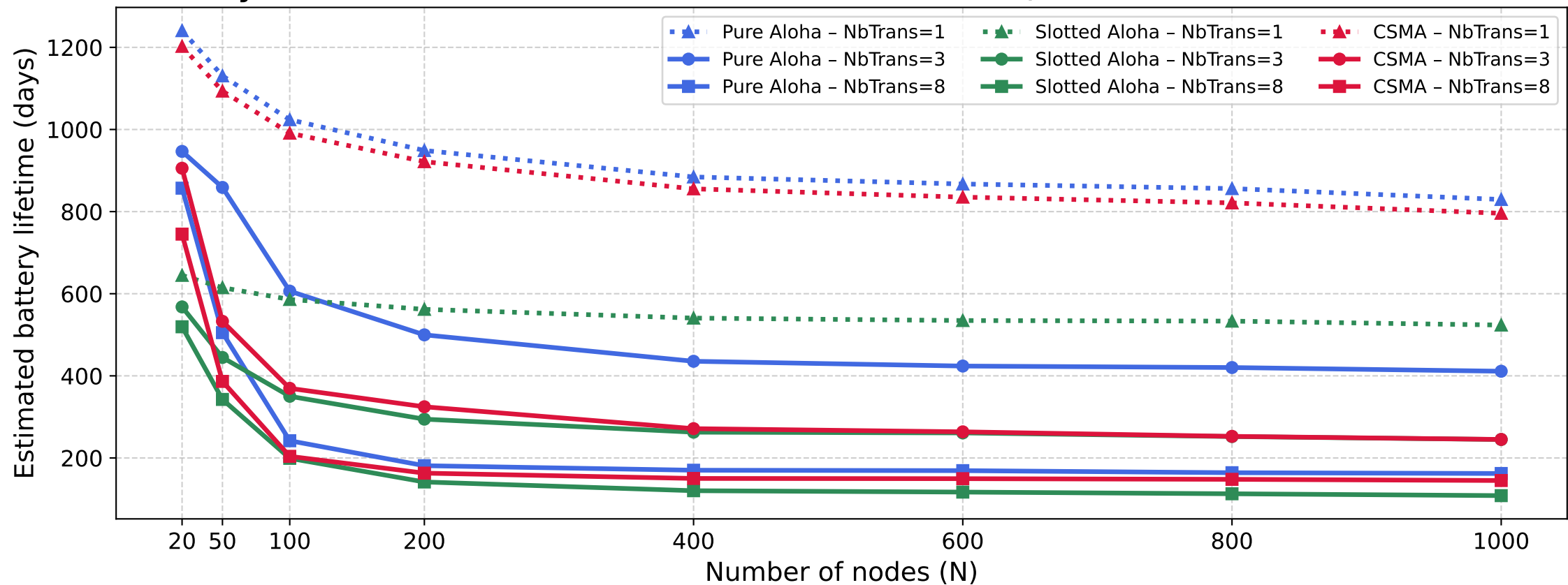
Battery Lifetime — Pure Aloha vs CSMA vs Slotted Aloha, Confirmed (NbTrans = 1 / 3 / 8)
