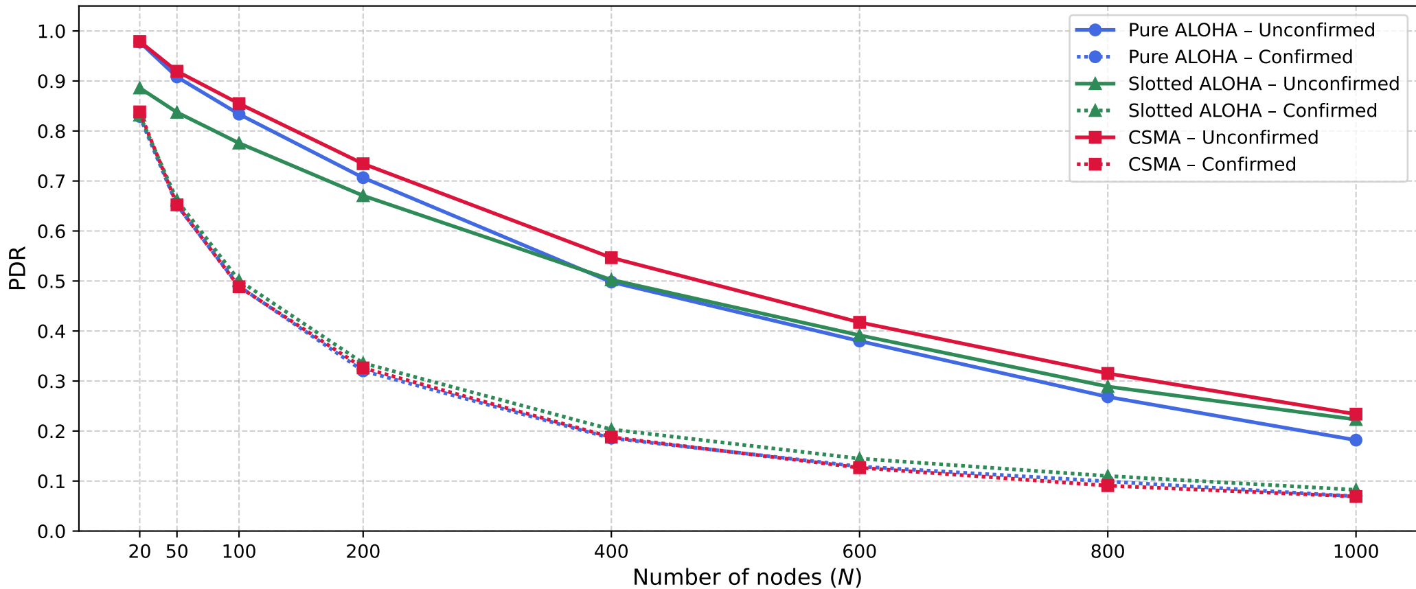
PDR — Pure ALOHA vs Slotted ALOHA vs CSMA (NbTrans=1)
