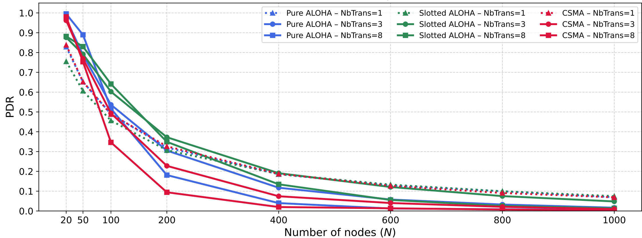
PDR — Pure ALOHA vs Slotted ALOHA vs CSMA, Confirmed (NbTrans = 1 / 3 / 8)
