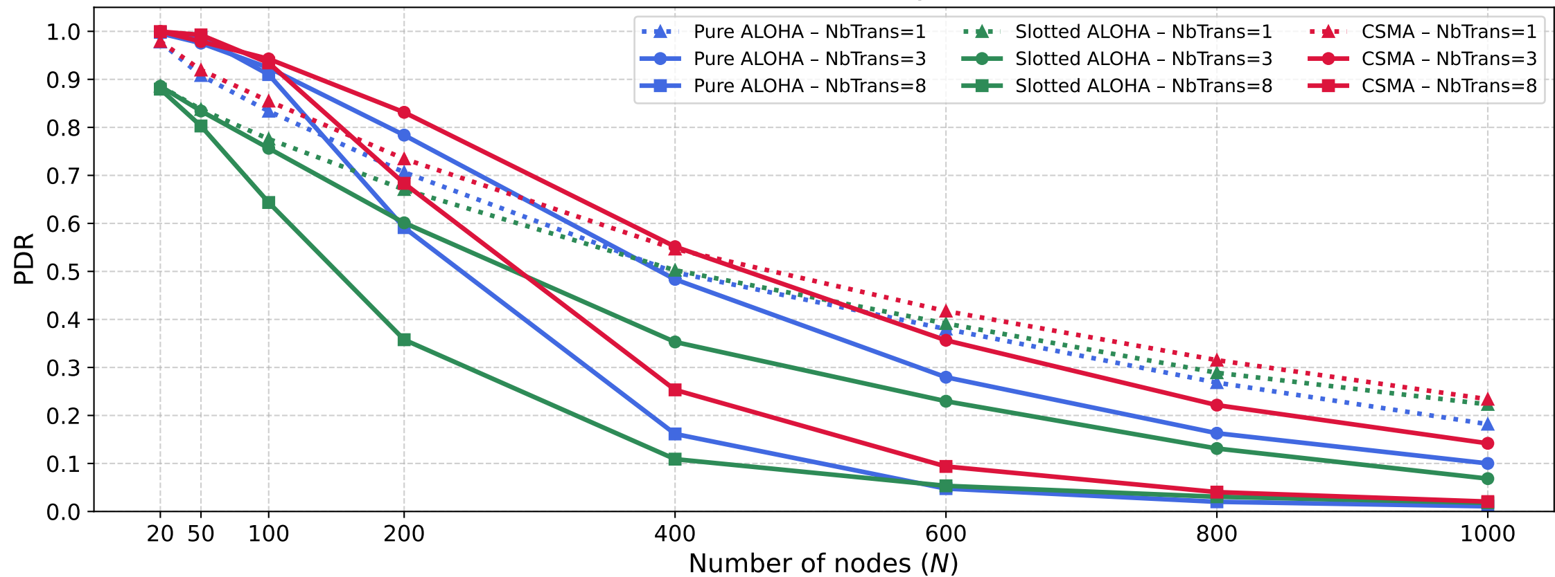
PDR — Pure ALOHA vs Slotted ALOHA vs CSMA, Unconfirmed (NbTrans = 1 / 3 / 8)
