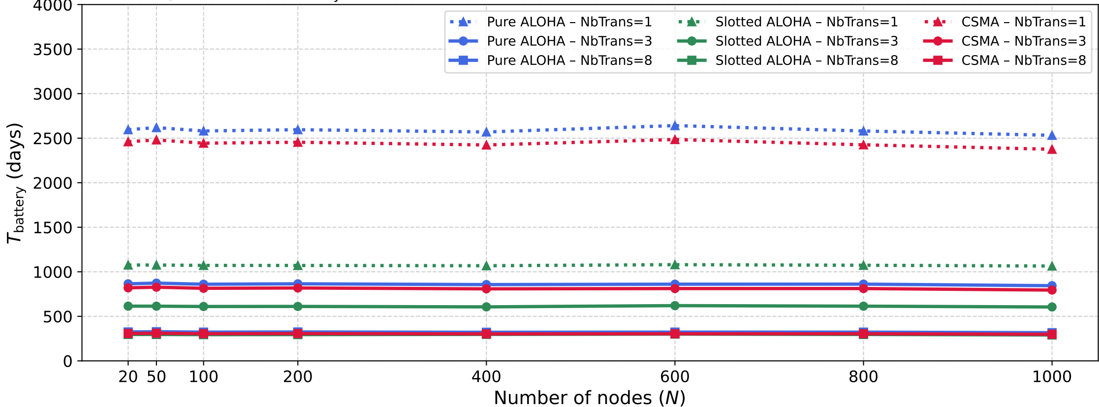
Estimated battery lifetime T_{\text{battery}} — Pure ALOHA vs Slotted ALOHA vs CSMA, Unconfirmed (NbTrans = 1 / 3 / 8)
