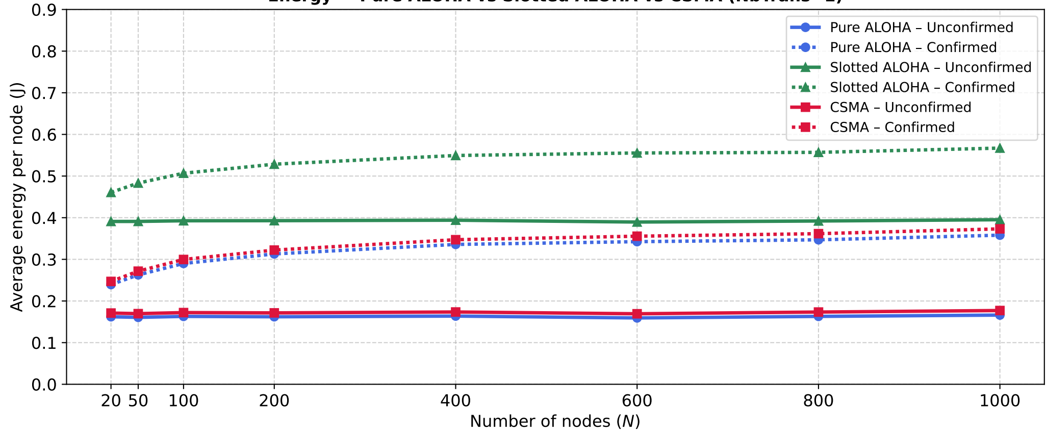
Energy — Pure ALOHA vs Slotted ALOHA vs CSMA (NbTrans=1)
