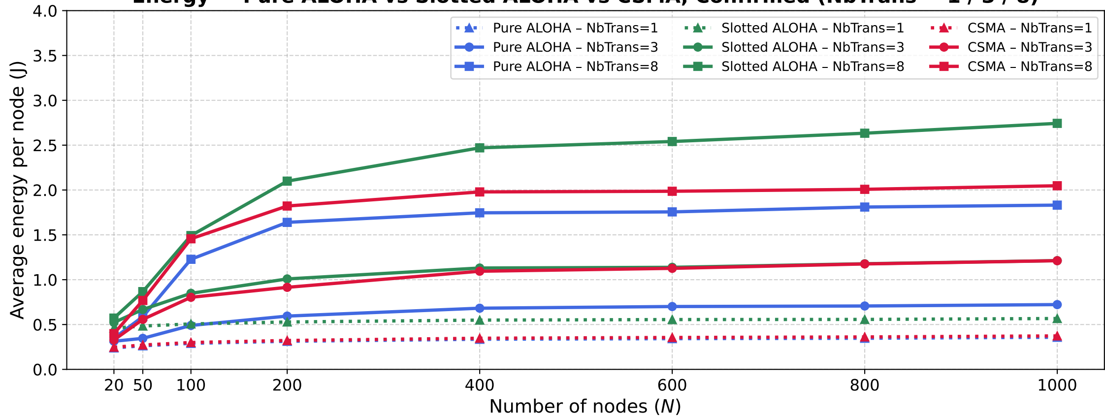
Energy — Pure ALOHA vs Slotted ALOHA vs CSMA, Confirmed (NbTrans = 1 / 3 / 8)
