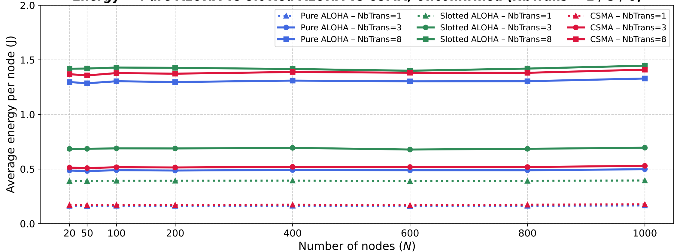
Energy — Pure ALOHA vs Slotted ALOHA vs CSMA, Unconfirmed (NbTrans = 1 / 3 / 8)
