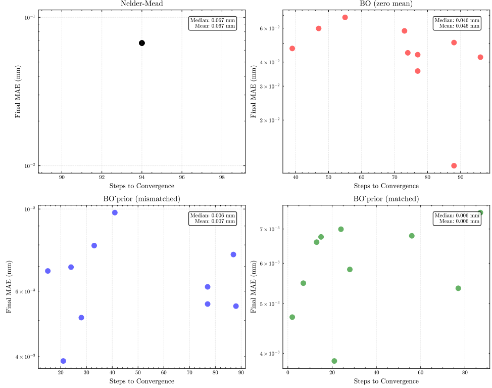
Figure 4.3: Final MAE versus steps to convergence for each trial. Fast convergence to a low error. Note the logarithmic y-axis.
