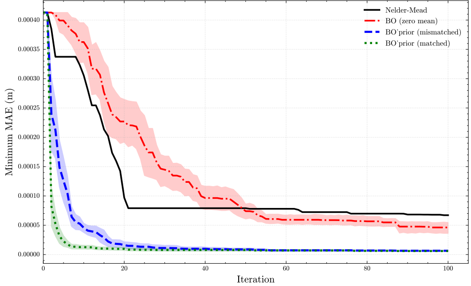
Figure 4.1: Convergence curve showing the cumulative minimum MAE over iterations for each optimization strategy.
