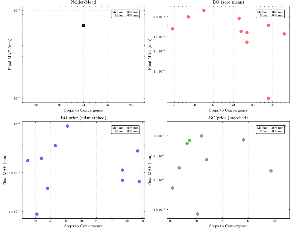
Figure 4.3: Final MAE versus steps to convergence for each trial, shown per method. Points in the bottom-left corner represent the ideal outcome: fast convergence to a low-error. Note the logarithmic y-axis.
