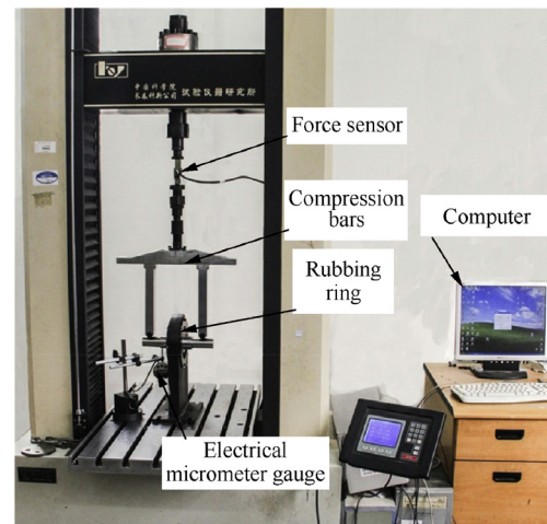
Fig. C1 Quasi-static test rig of rubbing ring.
