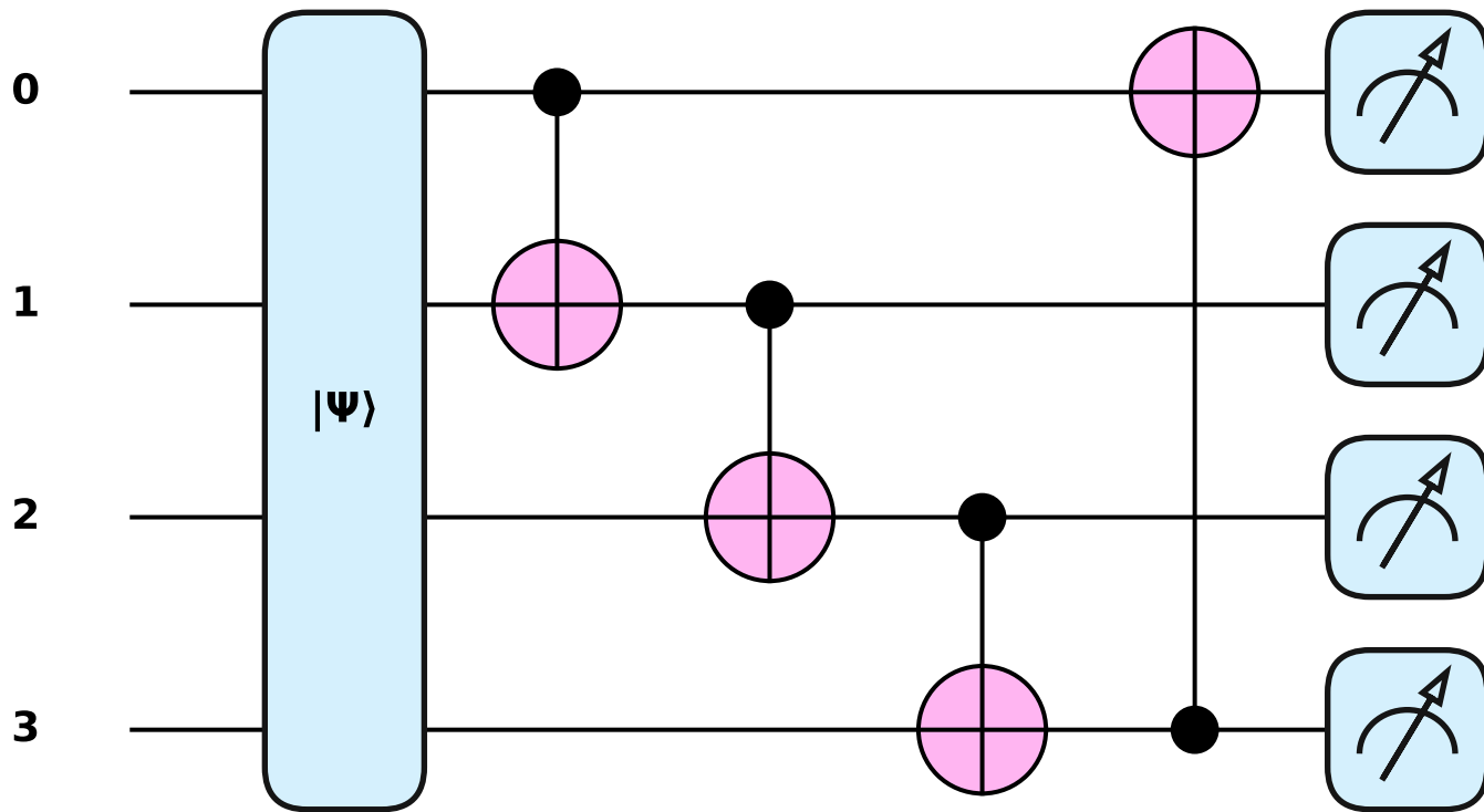
Amplitude encoding (16 pixels \rightarrow 4 qubits)
