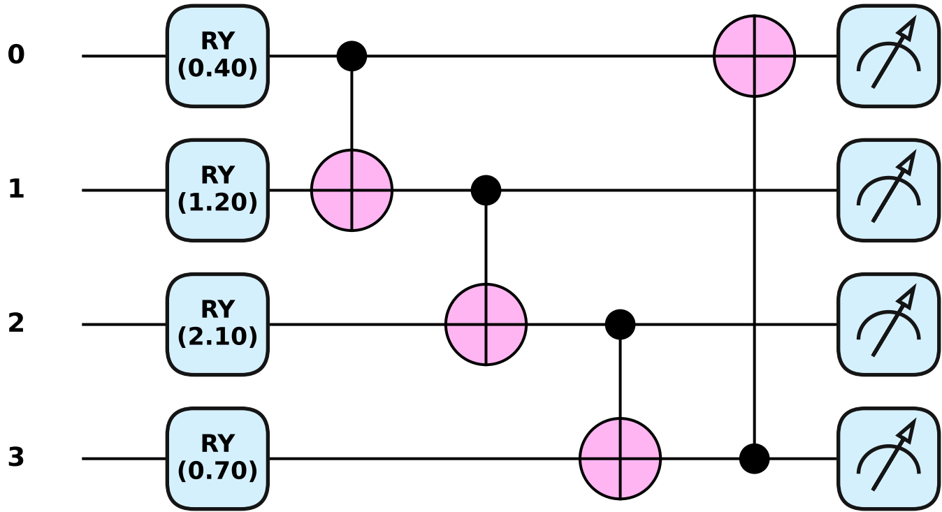
Angle encoding (qubit-per-pixel; 4-qubit illustration)
