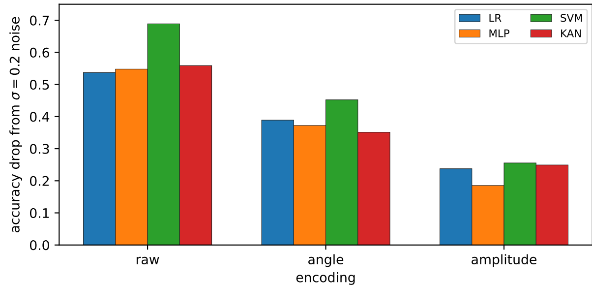
Robustness: lower is better
