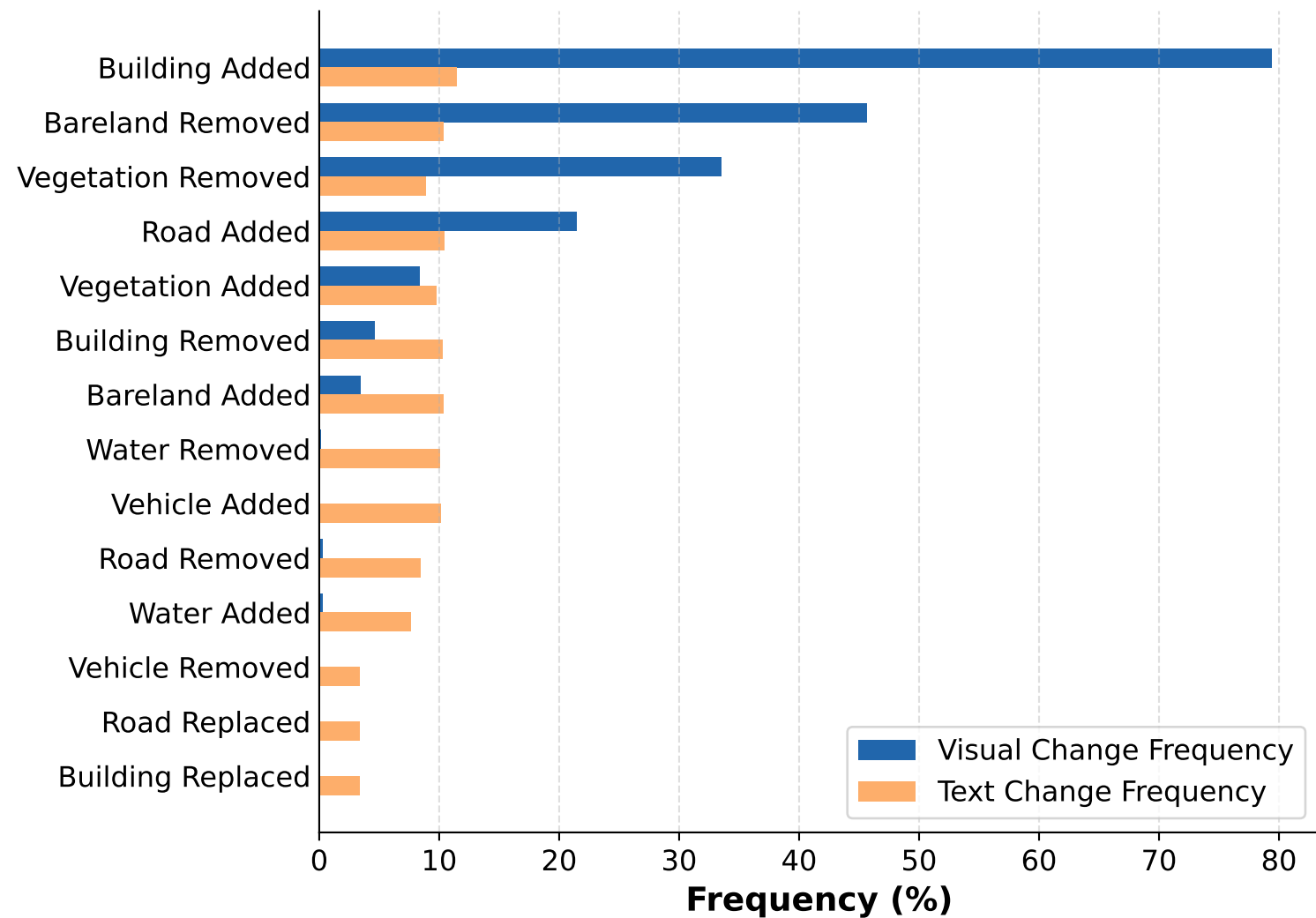
Global Change Frequency: Visual vs. Text
