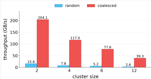
Whole GPU
