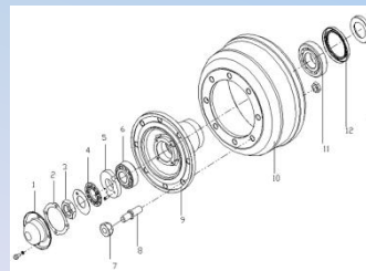
BRAKE DRUM CATAGORY I,II, & III
