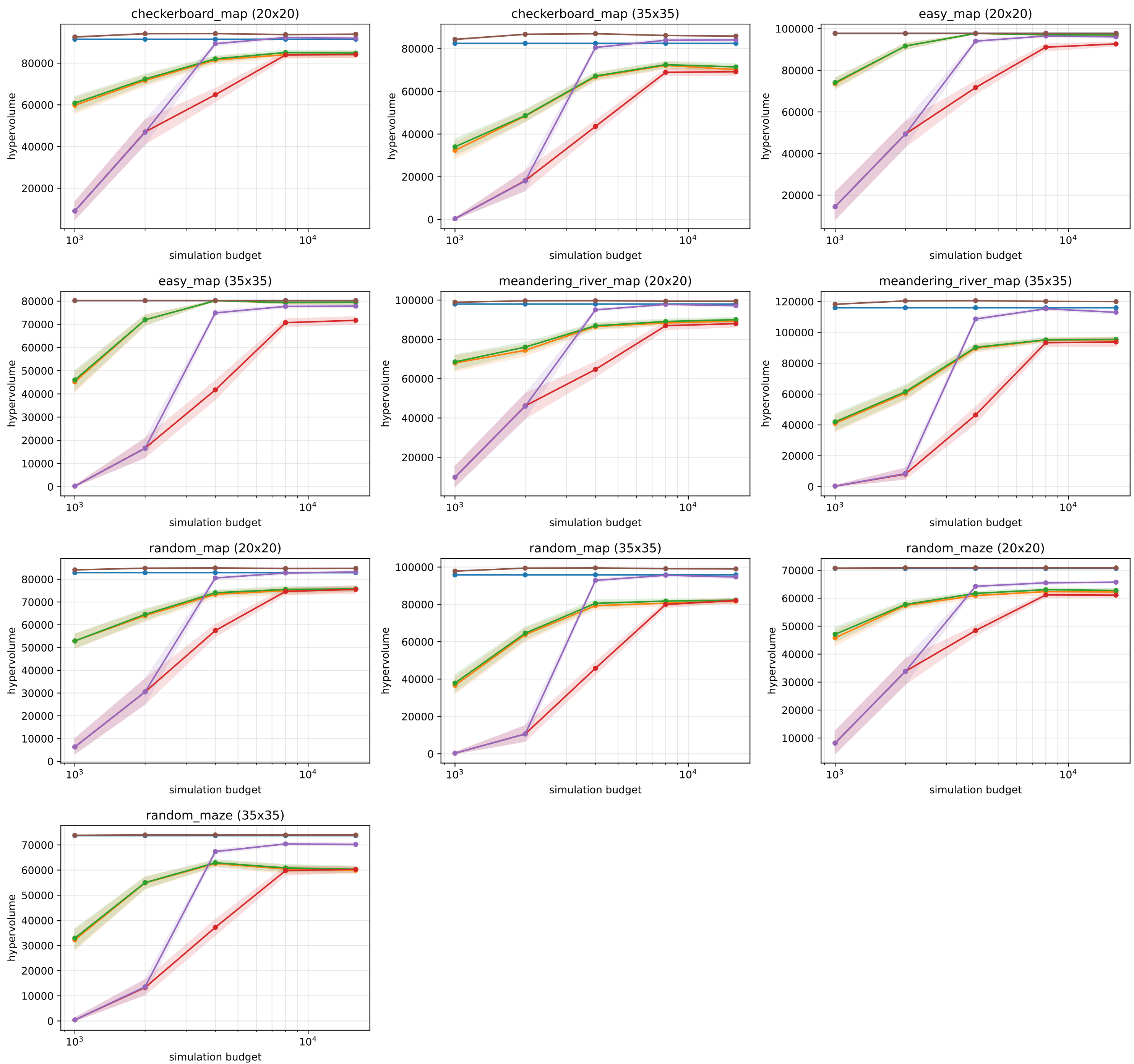
E2 anytime hypervolume (95% bootstrap CI)
