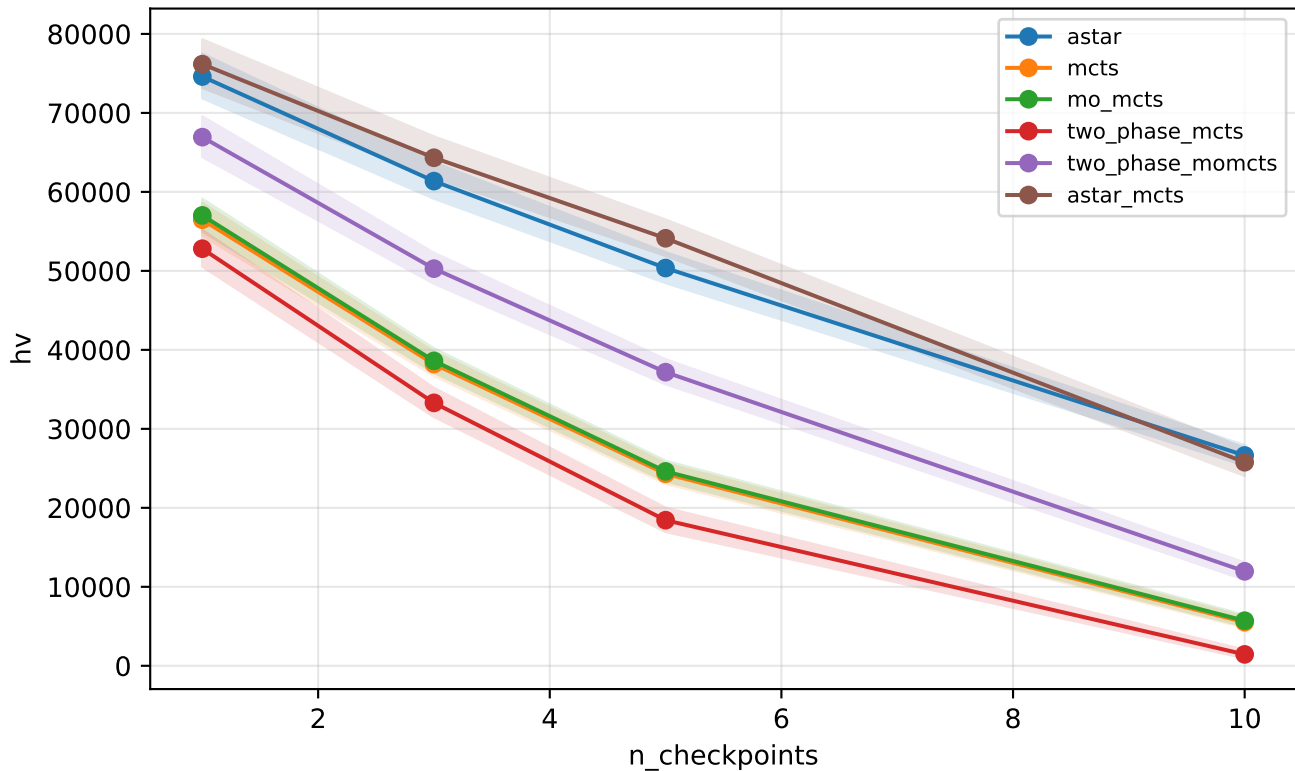
E4 HV vs number of checkpoints
