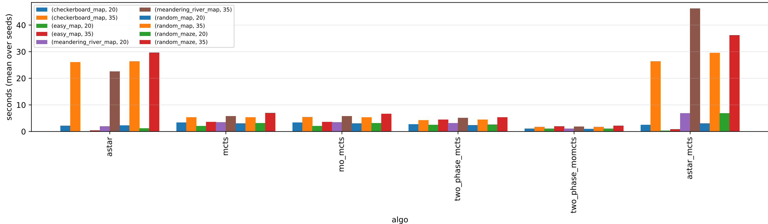
E1 wall-clock runtime per algorithm / map
