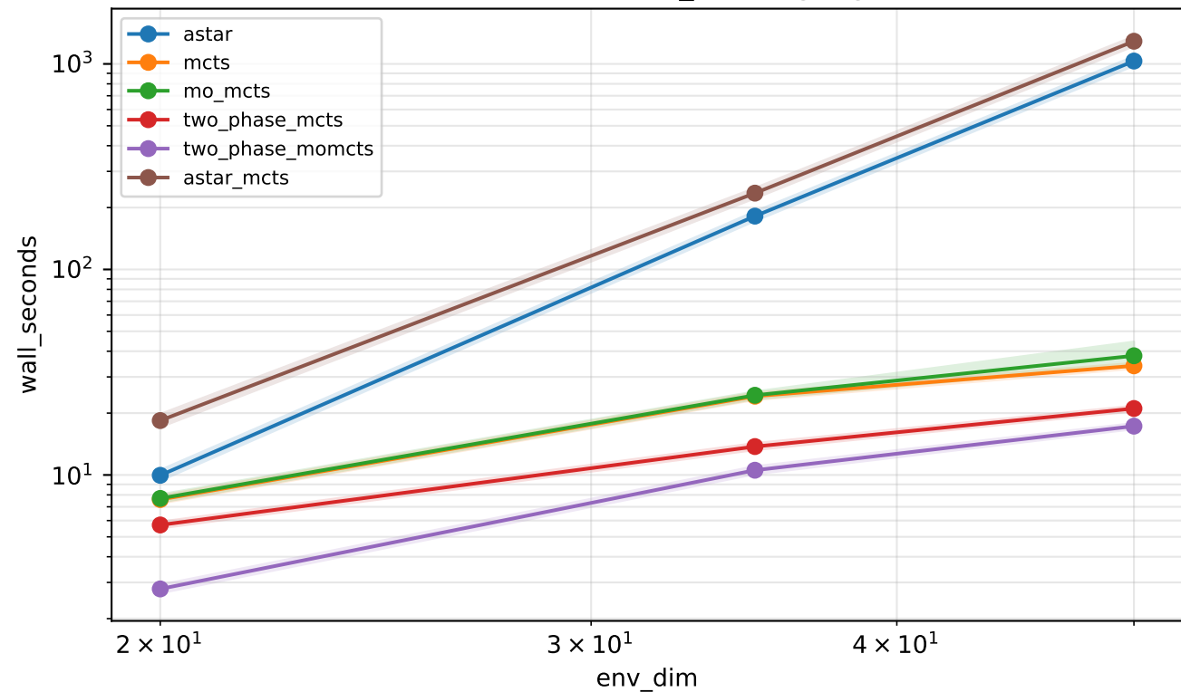
E4 runtime vs env_dim (log-log)
