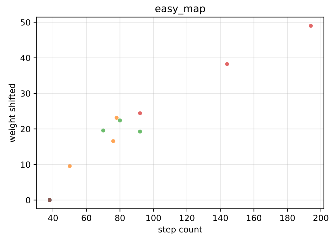
Pareto fronts (solved points) by algorithm — lower-left is better
