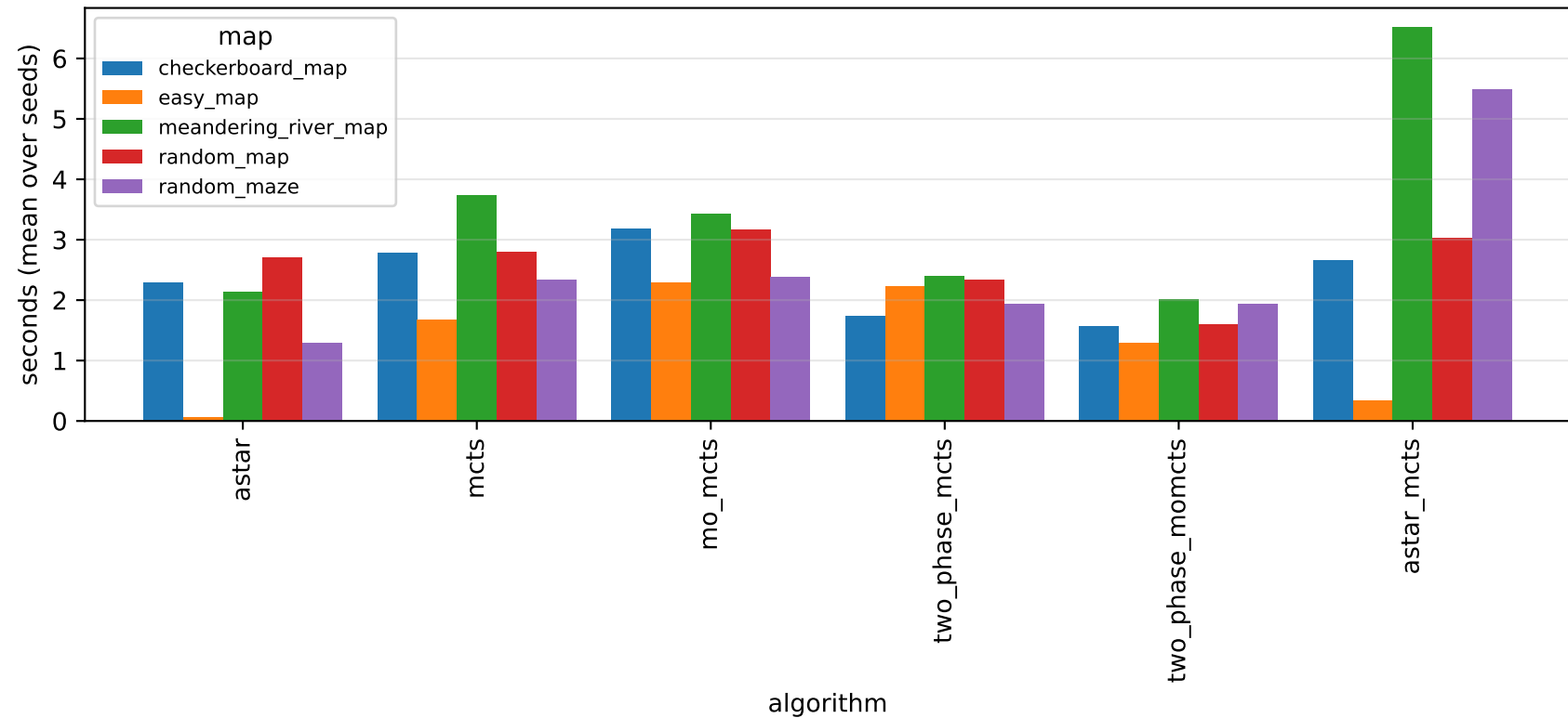
Wall-clock runtime per algorithm / map
