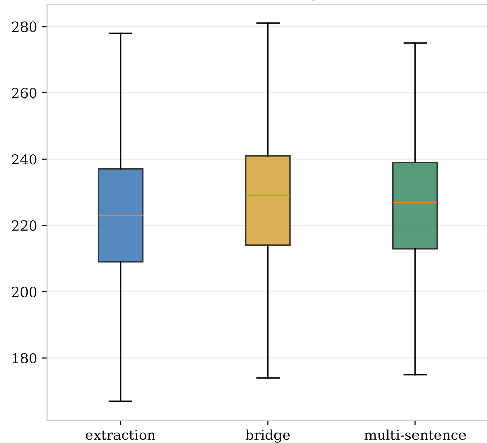
Context length
