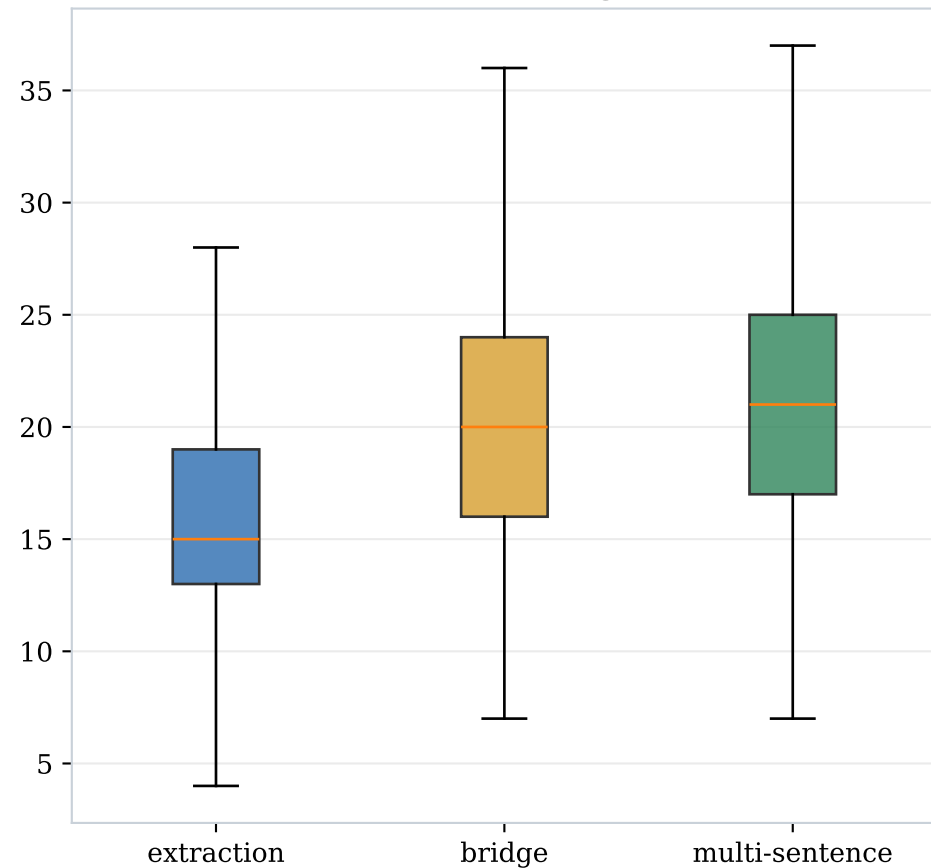
Question length
