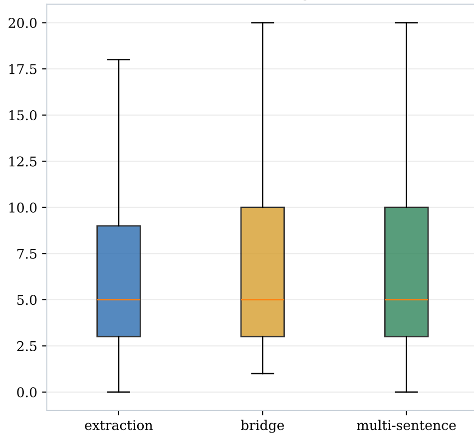
Answer length
