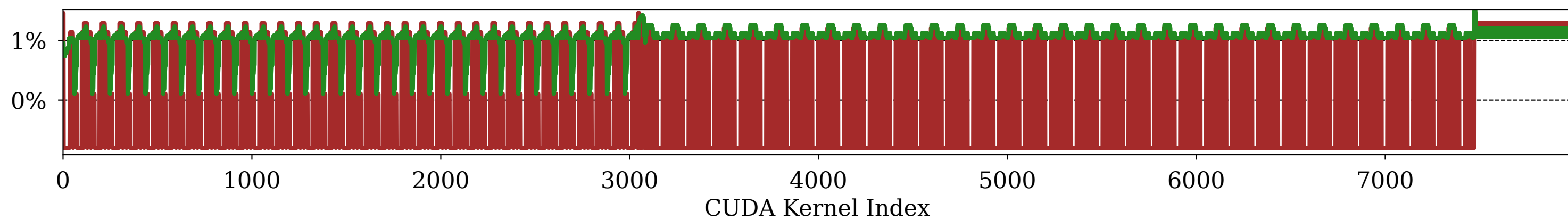
(b) ViT-512
