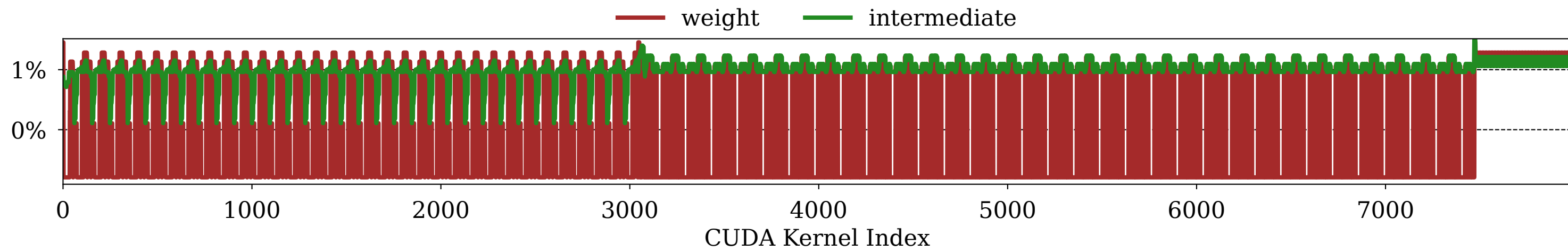
(a) BERT-128
