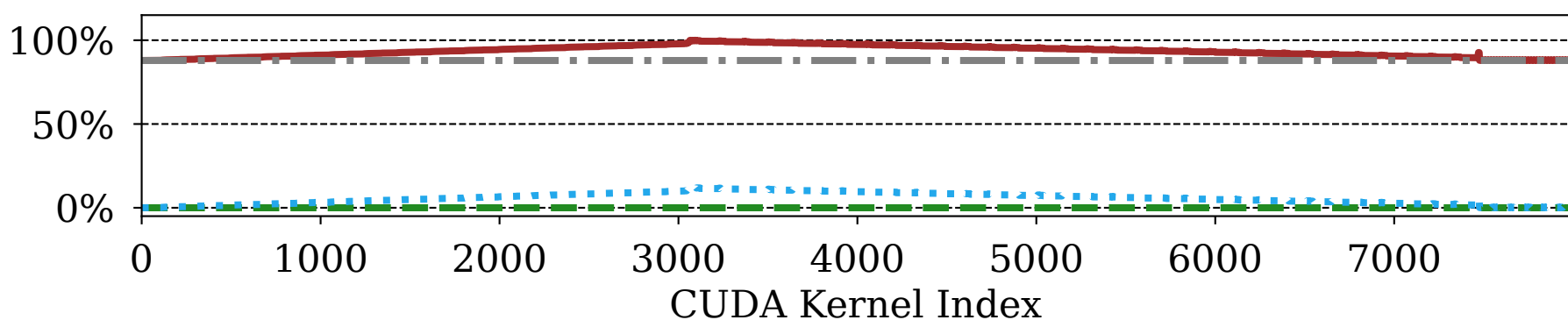
(c) Granite-3B-Instruct BS=1
