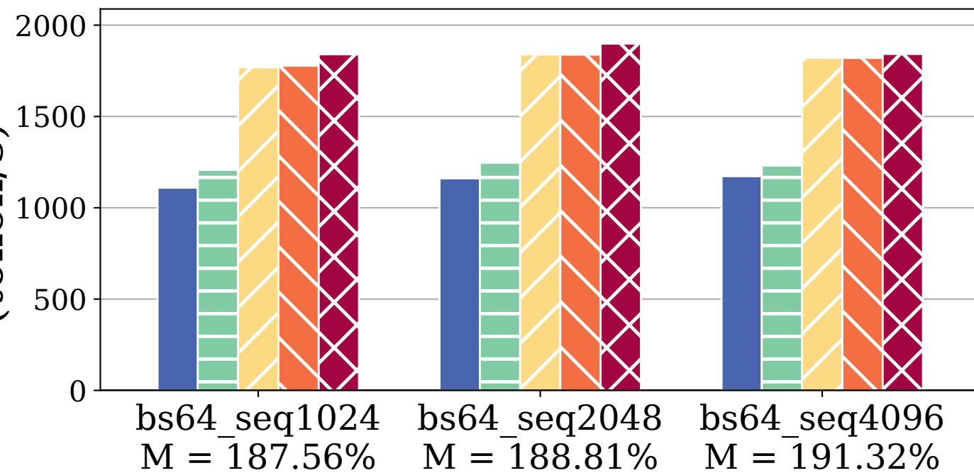
Training Throughput (token/s)
