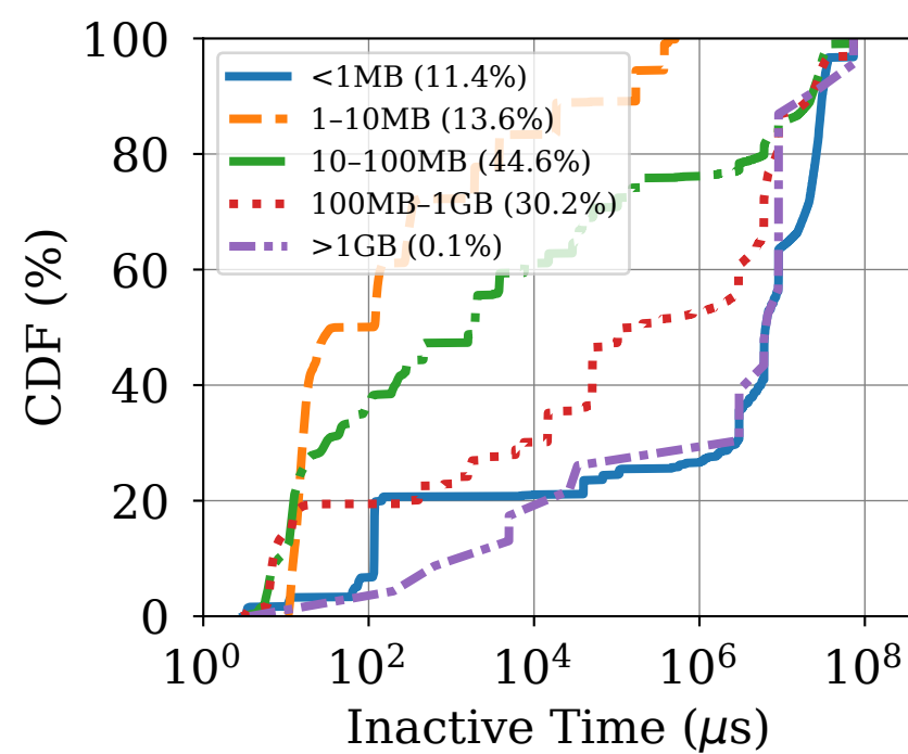
(b) GPT2-40B
