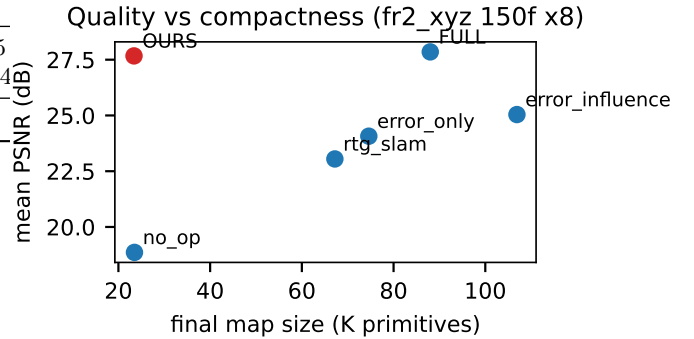
Figure 4: Quality vs compactness. OURS matches the ceiling at 3.8\times smaller map; all heuristic baselines bloat past 65k (fr2_xyz 150f \times 8).
