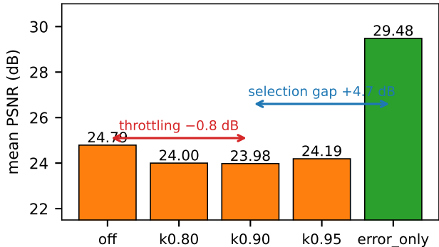
Decomposing the Replica gap (office0)
