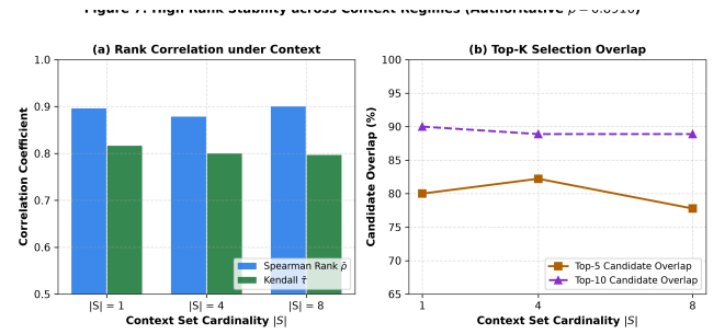
Figure 7: Rank Stability across Context Sizes |S| \in \{1, 4, 8\} . (a) Spearman \bar{\rho} \geq 0.8787 and Kendall \bar{\tau} \geq 0.7965 . (b) Top-5 candidate overlap averages 80.0%, proving rank invariance.
