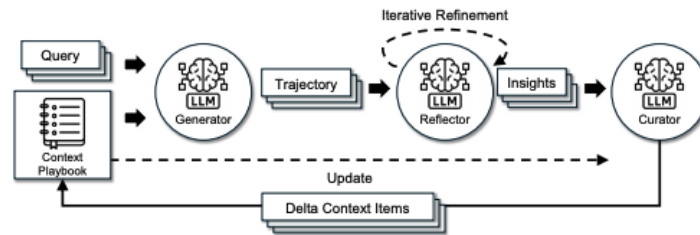
Figure 5: ACE framework
