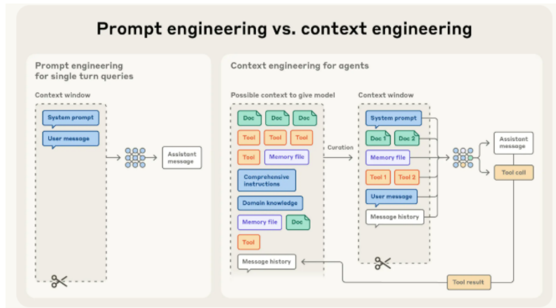
Figure 3: Context engineering
