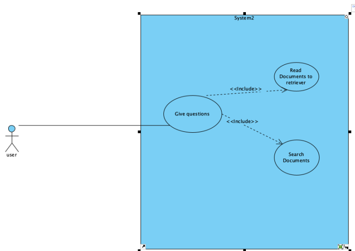
Figure 7: Usecase Diagram
