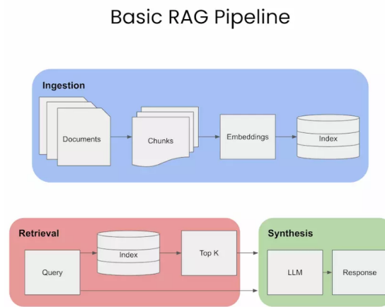
Figure 1: RAG architecture
