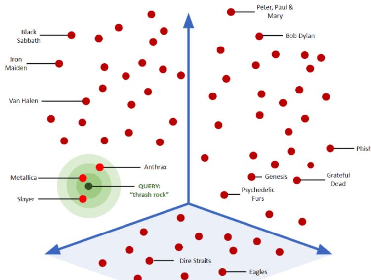
Figure 6: Vector search
