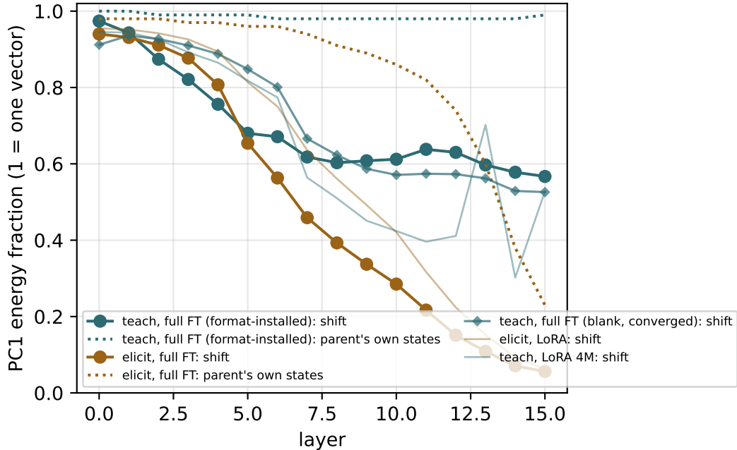
is the task shift one direction?
