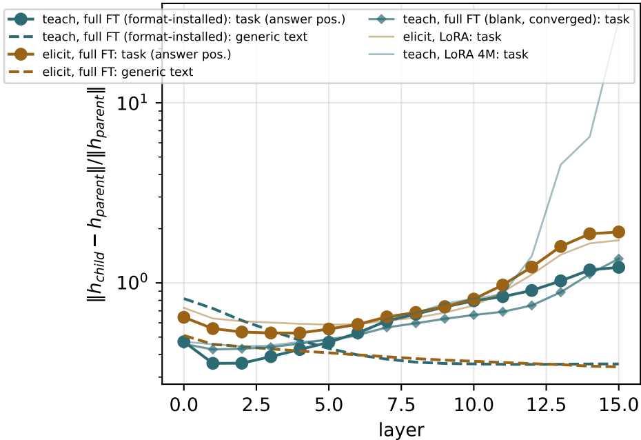
relative residual shift
