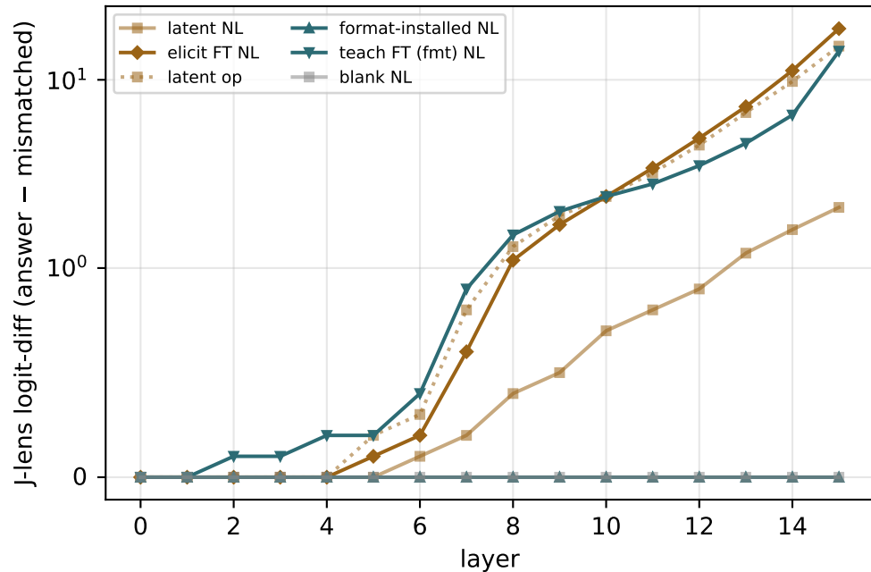
answer-specific signal by depth
