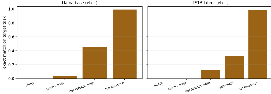
Figure 7: Donor patching on two elicit parents (weights frozen except the last bar): direct, mean vector, per-prompt states, and the fine-tuned child for scale; the self-chain bar is the construction check of Table 1, not a patch.
