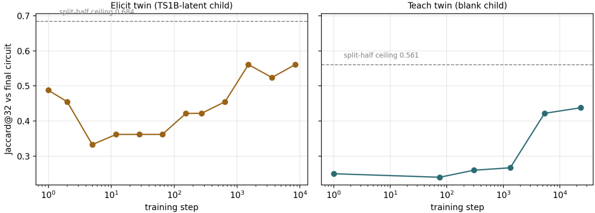
Figure 2: Circuit formation, elicit (left) vs teach (right); dashed = split-half ceiling.
