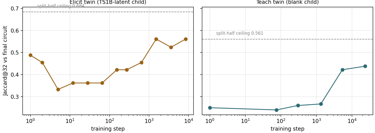
Figure 1: Circuit formation, elicit (left) vs teach (right); dashed = split-half ceiling.
