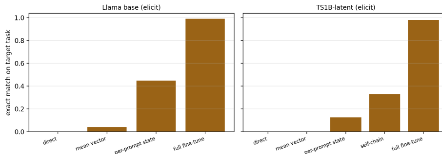
Figure 5: Donor patching on the elicit parent (right; left: the same on Llama-3.2-1B, the second elicit parent of M13–M17), weights frozen except the last bar: unpatched parent, mean vector, per-prompt states, and the fine-tuned child for scale.
