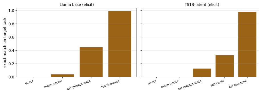
Figure 5: Donor patching on the elicitor parent (right; left: the same on Llama-3.2-1B, the second elicitor parent of M12–M16), weights frozen except the last bar: unpatched parent, mean vector, per-prompt states, and the fine-tuned child for scale.
