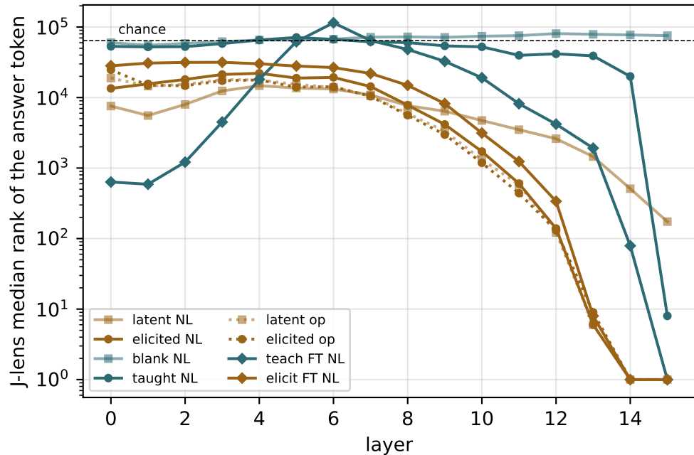
is the answer in J-space?
