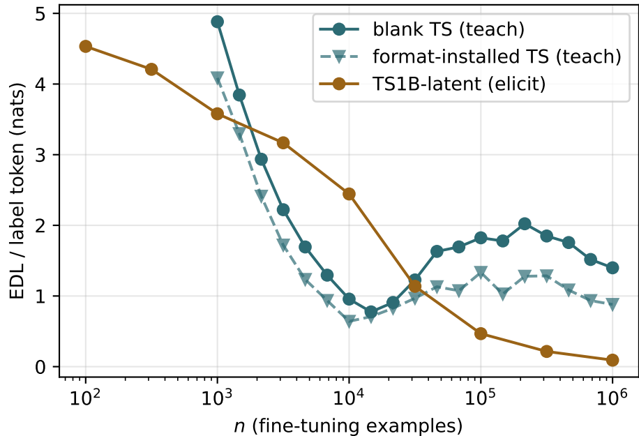
Learning-curve signature
