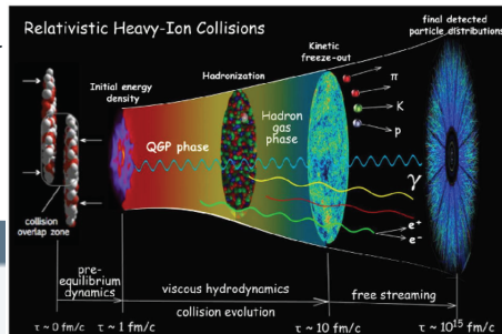
Schematic evolution of a relativistic heavy-ion collision. Adapted from Purdue RCAC News (2023).
