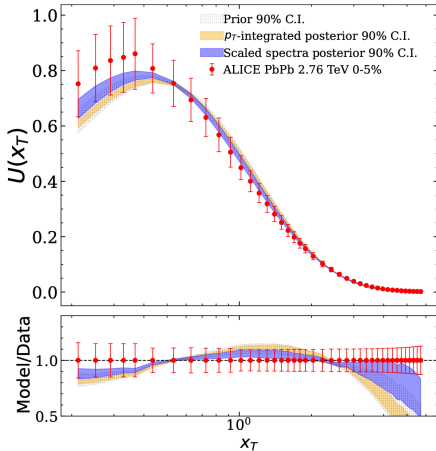
Identified-particle spectra collapse onto a universal curve after rescaling. Domingues & Luzum, arXiv:2603.15891 (2026).
