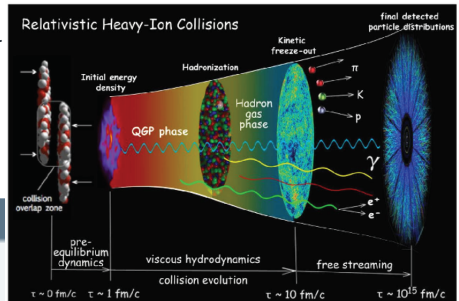
Schematic evolution of a relativistic heavy-ion collision.
