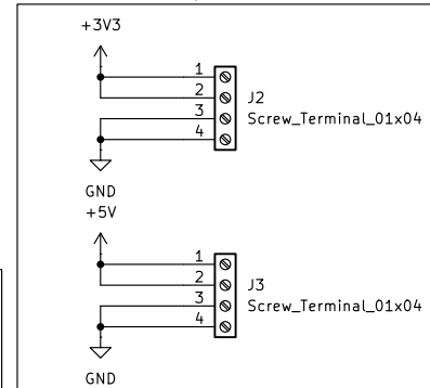
Output Connector
