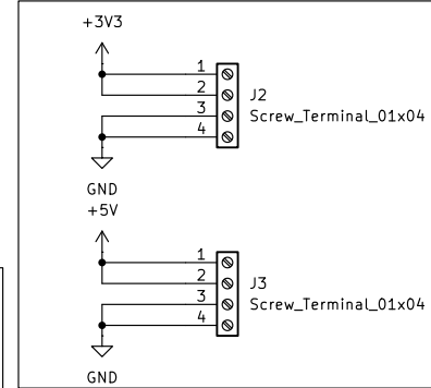
Output Connector
